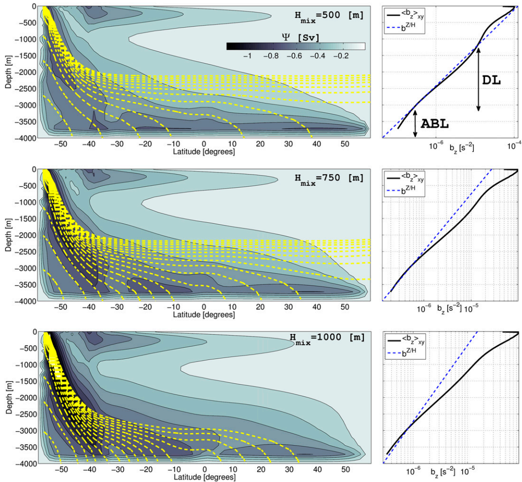
FIG. 9. As in Fig. 7, but for the sensitivity of MOC to vertical decay scale H_{mix} . The diffusivity \kappa_b = 3 \times 10^{-4} \text{ m}^2 \text{ s}^{-1} for all three cases, while H_{mix} changes from 500 m (top) to 1000 m (bottom). Note that the top panel is the same as the middle panel in Fig. 7.
